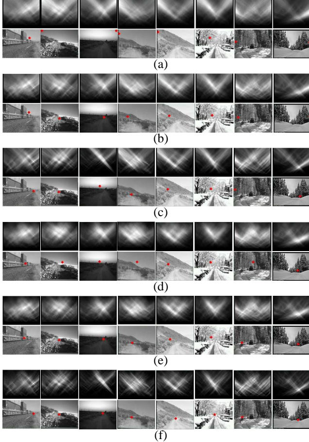
Fig. 10. Comparison of vanishing point estimation based on different combinations: (a) ‘‘Hard’’+‘‘Global’’; (b) ‘‘Soft’’+‘‘Global’’; (c) ‘‘Soft’’+‘‘Global’’ ( T>0.3 ); (d) ‘‘Hard’’+‘‘Local’’; (e) ‘‘Soft’’+‘‘Local’’; (f) ‘‘Soft’’+‘‘Local’’ ( T>0.3 )
