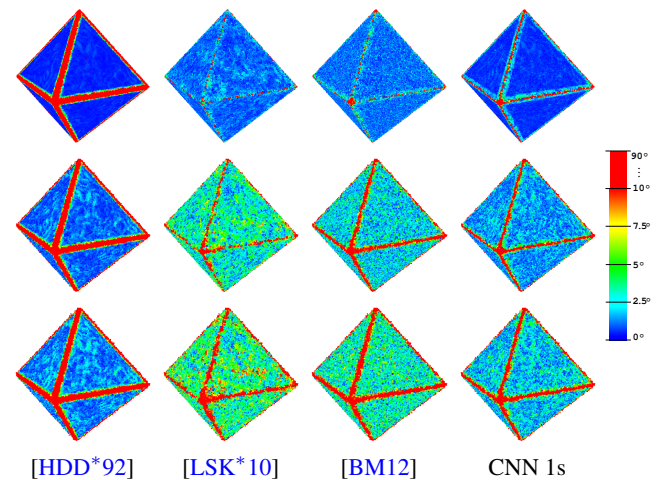
Figure 11: Visual results of four estimation algorithms on an octahedron (100k points) with 50% noise (top line), 150% noise (middle) and 200% noise (bottom). Color scale, given on the right, maps a deviation angle to a color (red is a deviation greater than 10^\circ ).
