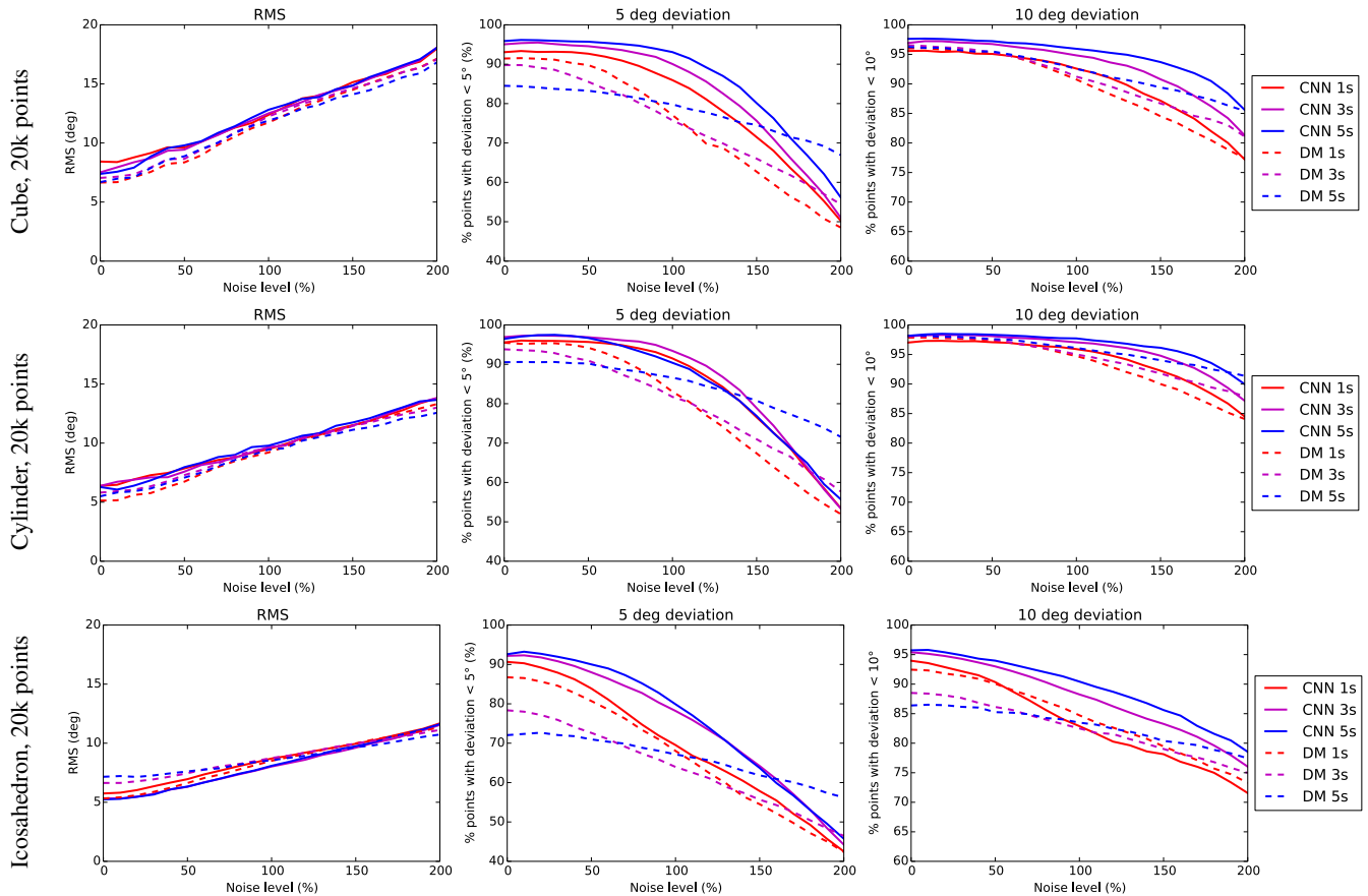
Figure 10: Comparison of our method (CNN) and a similar CNN estimation based on depth map input (DM) with multiscale ( m s).
