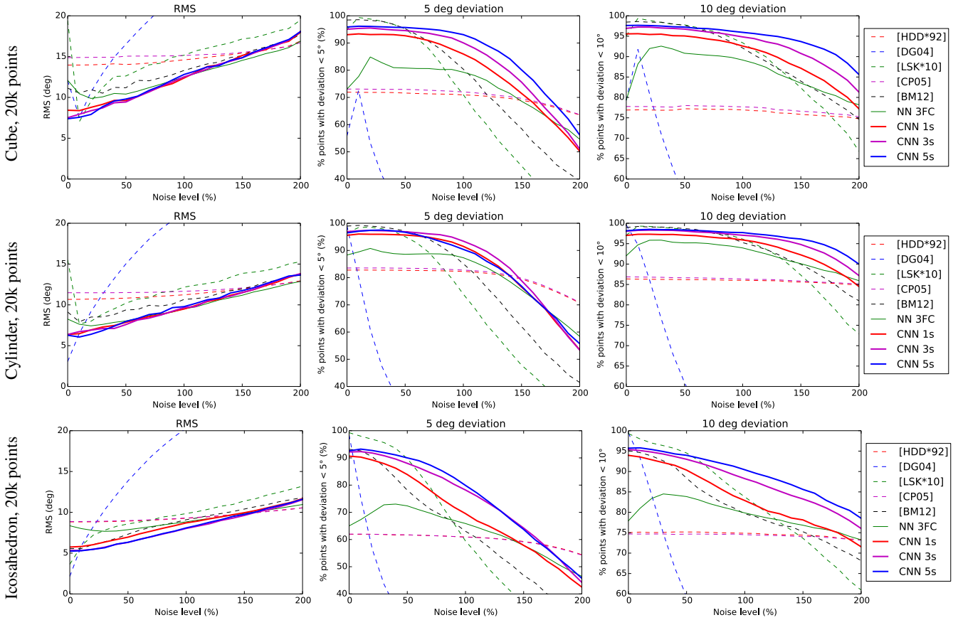
Figure 9: Comparison of various methods on simple geometric models with varying Gaussian noise (standard deviation expressed a % of the mean distance between points) and no density variation. NN 3FC: network with 3 fully-connected layers on the same Hough image-accumulator as ours; CNN n s: our method with n scales.
