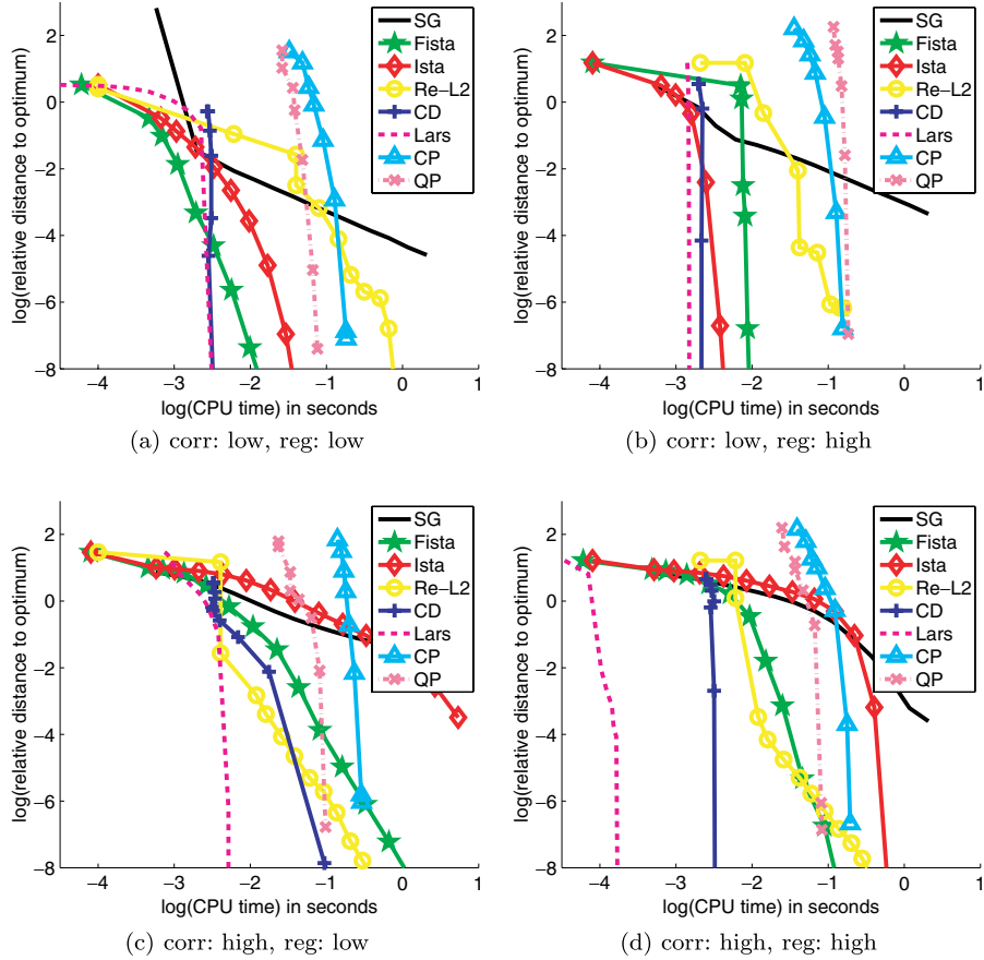
Fig. 8.1. Benchmark for solving the Lasso for the small-scale experiment ( n = 200 , p = 200 ), for the two levels of correlation and two levels of regularization, and eight optimization methods (see main text for details). The curves represent the relative value of the objective function as a function of the computational time in second on a \log_{10}/\log_{10} scale.
