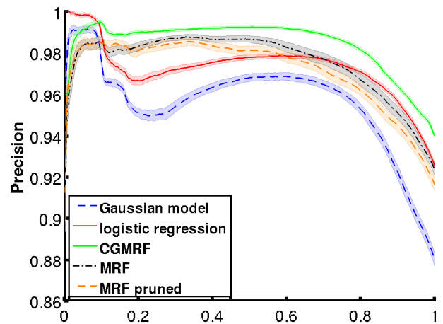
Figure 8.3: Precision coverage curves on Sevrans. Averaged precision coverage curves for the inference for 300 random resamplings of 7% of revealed labels on the city of Sevrans. Shaded areas represent one standard deviation. (Best seen in color.)
