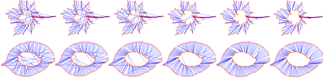
Fig. 3. This figure shows the evolution of context-dependent silhouette matching on the Swedish set, for different and increasing values of \alpha . We clearly see that when \alpha increases the matching results are better. We set \beta = 0.1 and t = 1 .
