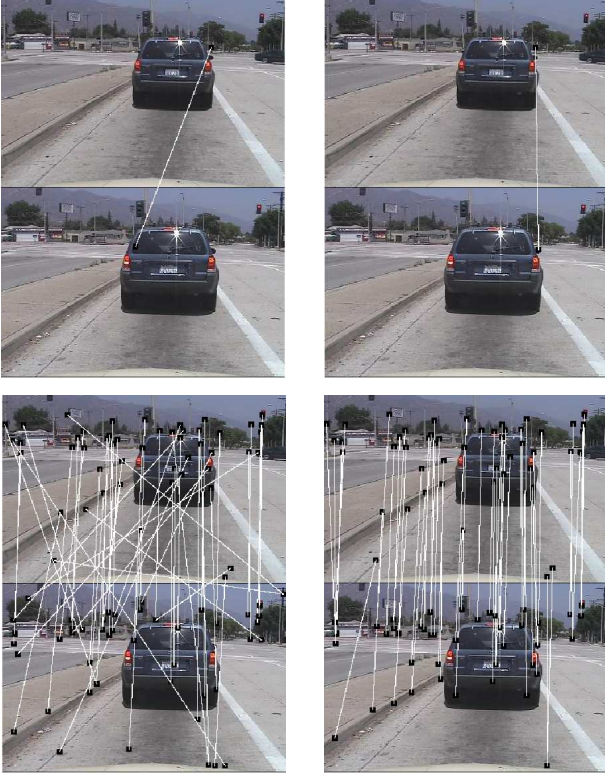
Fig. 2. This figure shows a comparison of the matching results when using a naive matching strategy without geometry and our “context-dependent” kernel matching. (Top figures) show the distribution of the kernel values k(x_i, x_j), j \in \mathcal{I}_q using a context-free kernel (left) and our “CDK” kernel (right). We can clearly see that the highest value changes its location so the matching results are now corrected (as shown in middle figures). (Bottom) other matching results.
