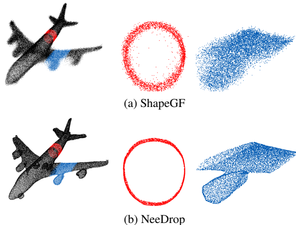
Figure 12. Comparing the point cloud generated by ShapeGF to a point cloud (of the same size) sampled on our generated mesh.
