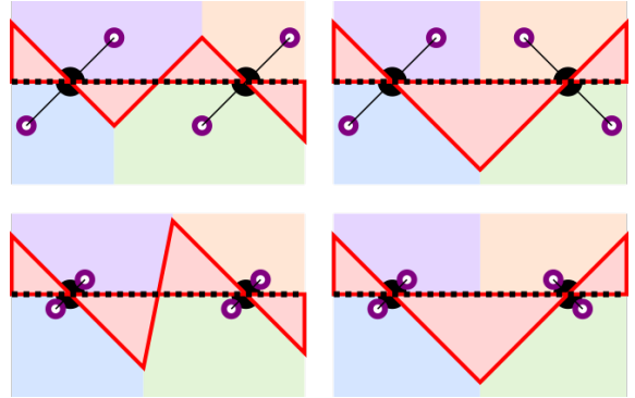
(a) No point belonging to P_{\text{same}} .
